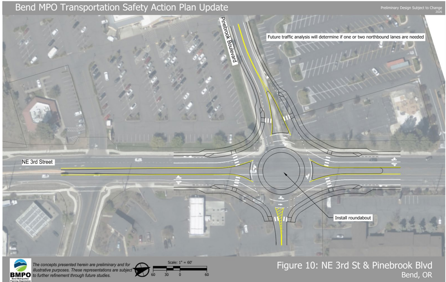
Figure 10. 3rd Street / Pinebrook Boulevard Treatments
