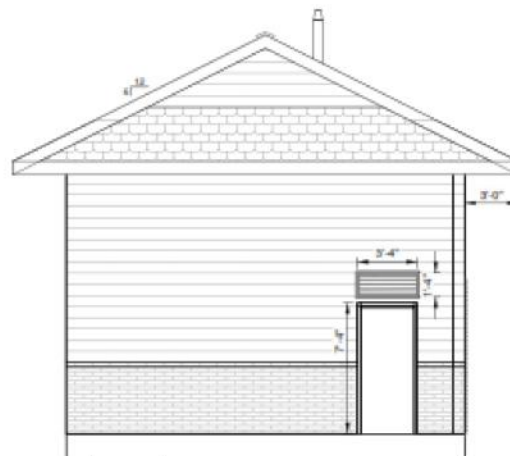
GENERATOR BUILDING WEST ELEVATION SCALE: 1/2"=1'-0"
