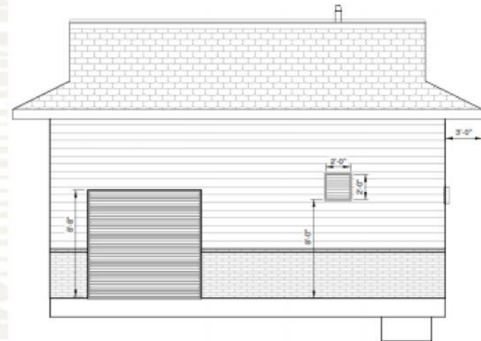
GENERATOR BUILDING SOUTH ELEVATION SCALE: 1/2"=1'-0"
