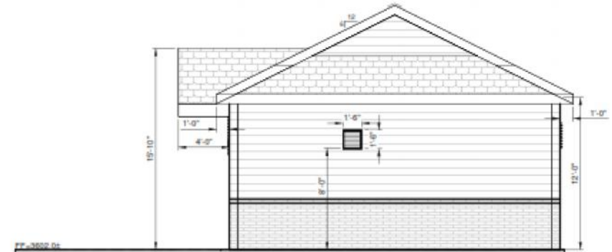
LIFT STATION EAST ELEVATION SCALE: 1/2"=1'-0"
