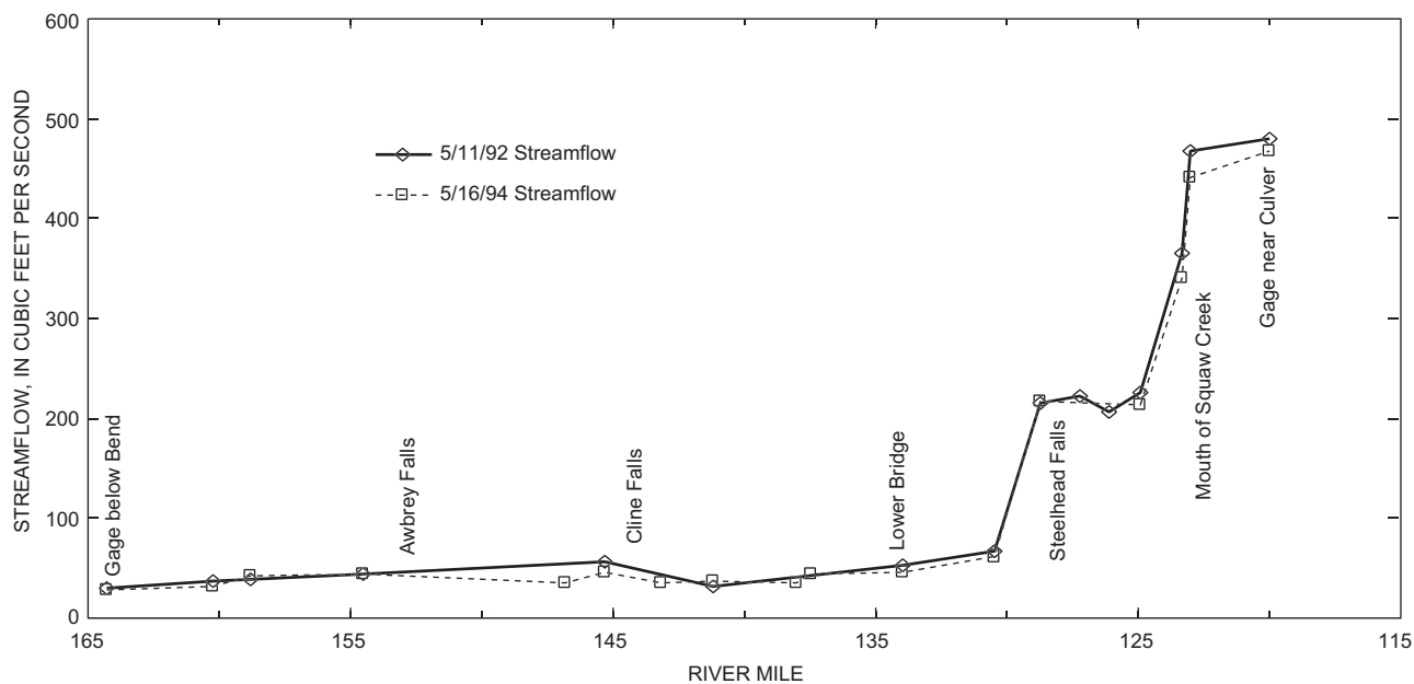
Figure 17. Gain in flow of the Deschutes River, Oregon, due to ground-water discharge between river miles 165 and 120, May 1992 and May 1994. (Some of the gain is due to ground-water discharge along the lower 2 miles of Squaw Creek.)
