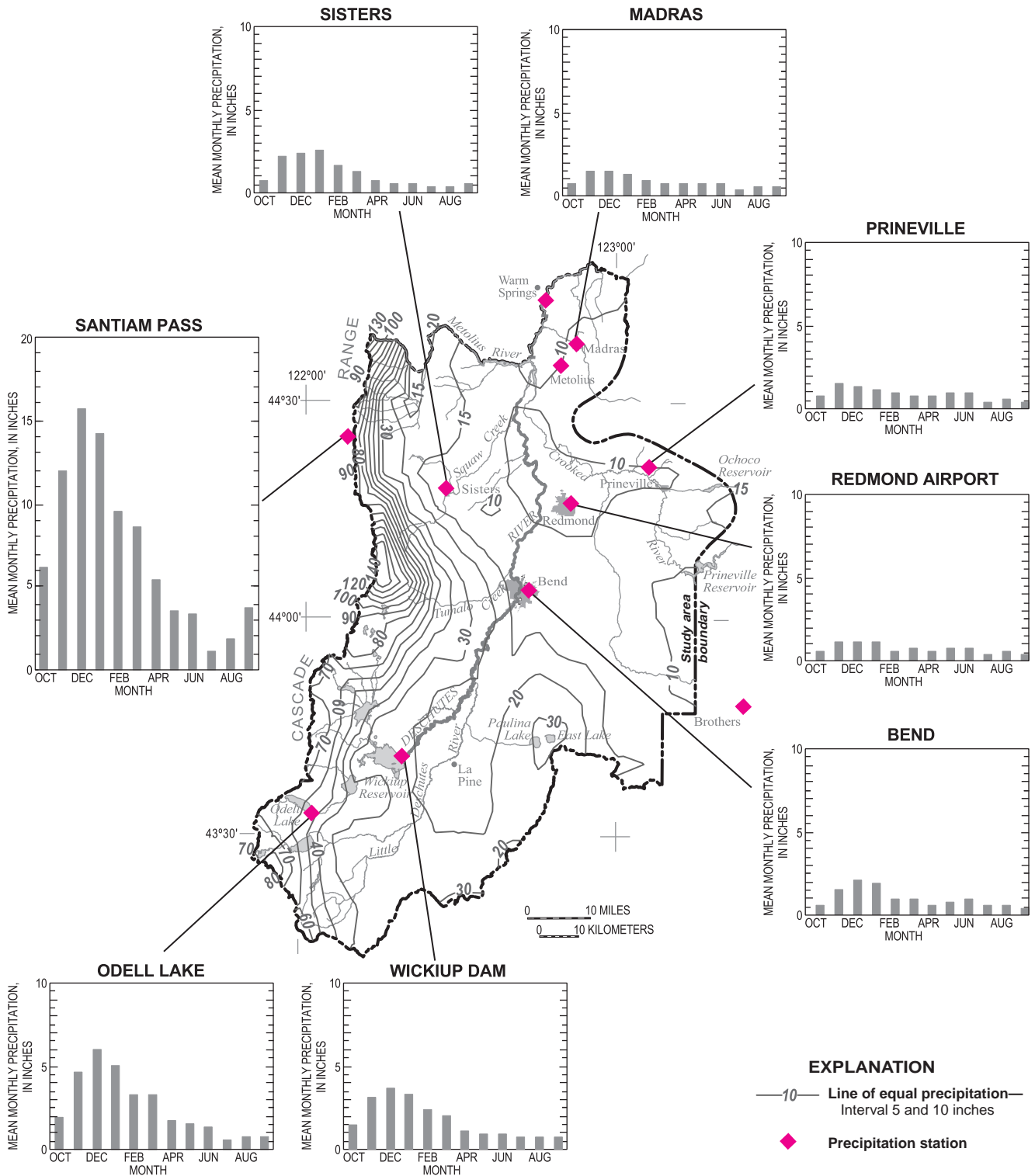
Figure 3. Lines of equal precipitation and graphs of mean monthly precipitation for selected precipitation stations in the upper Deschutes Basin, Oregon.
