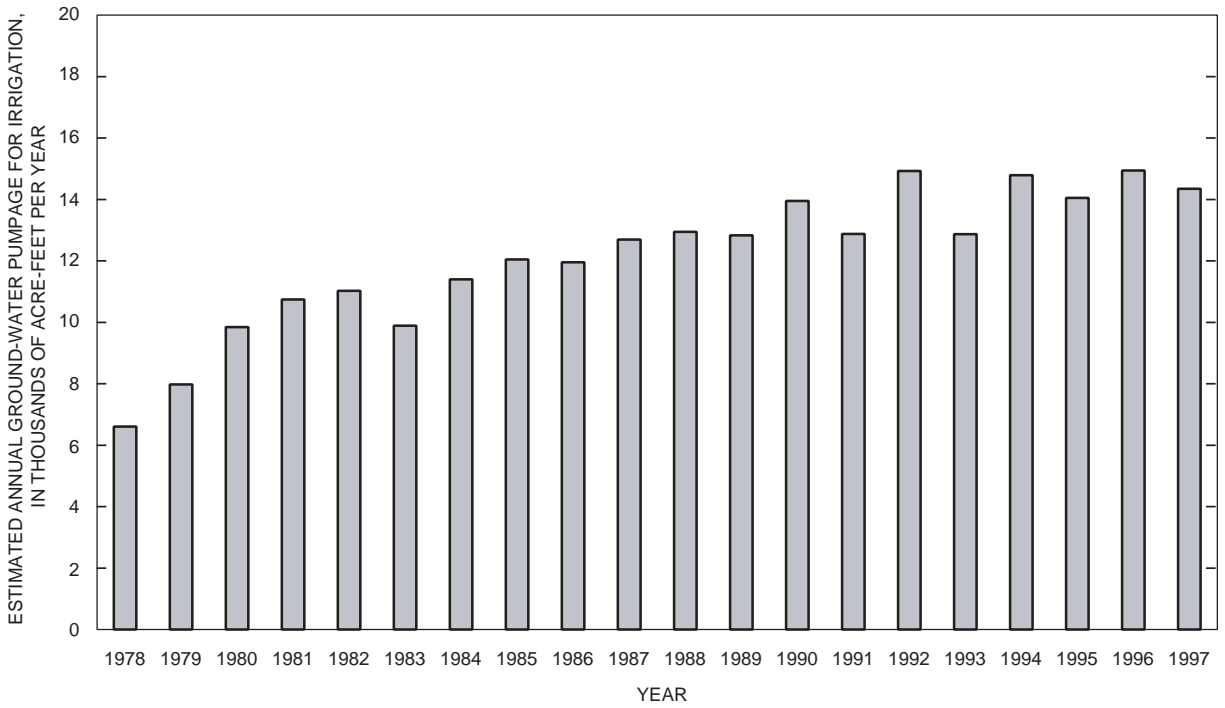
Figure 24. Estimated annual ground-water pumpage for irrigation in the upper Deschutes Basin, Oregon, 1978–97.
