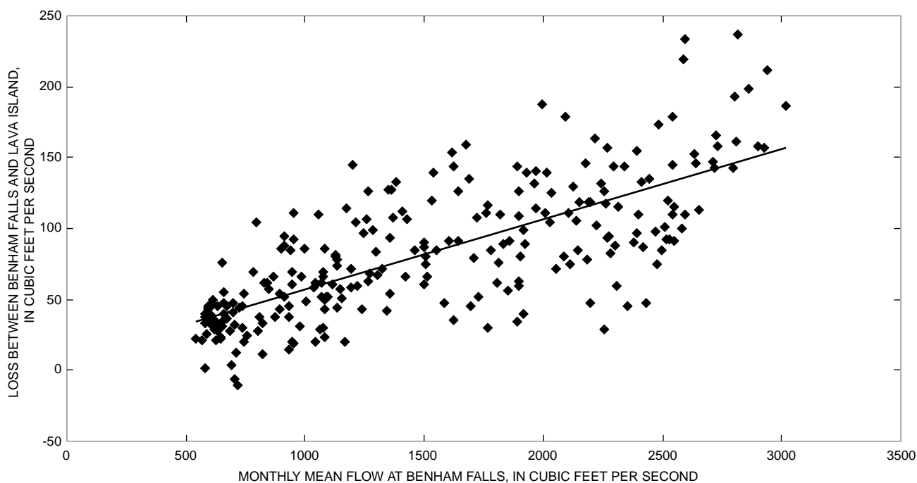
Figure 13. Relation between monthly mean losses along the Deschutes River between Benham Falls and Lava Island and flow at Benham Falls.
