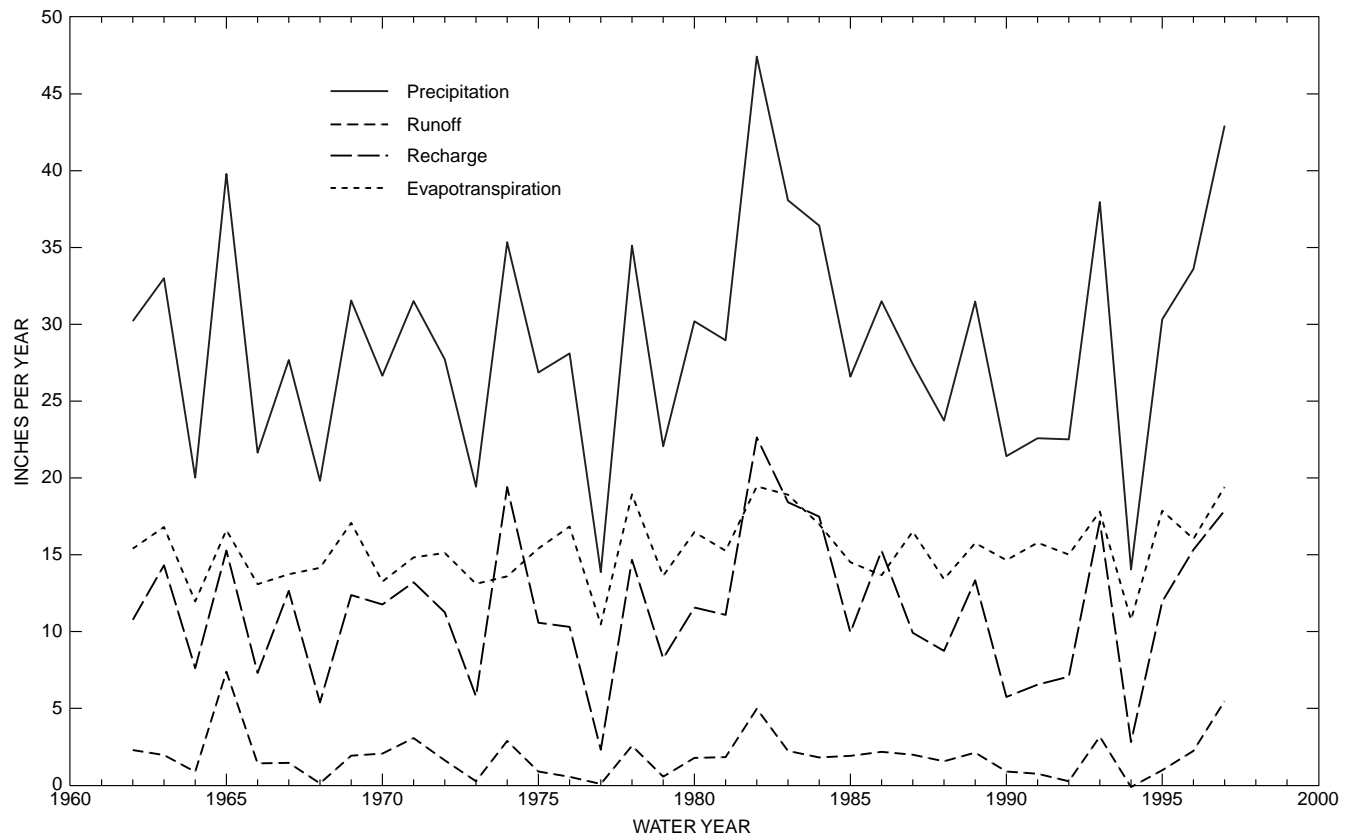
Figure 7. Annual mean components of the basinwide water budget, estimated using the Deep Percolation Model for water years 1962–97.
