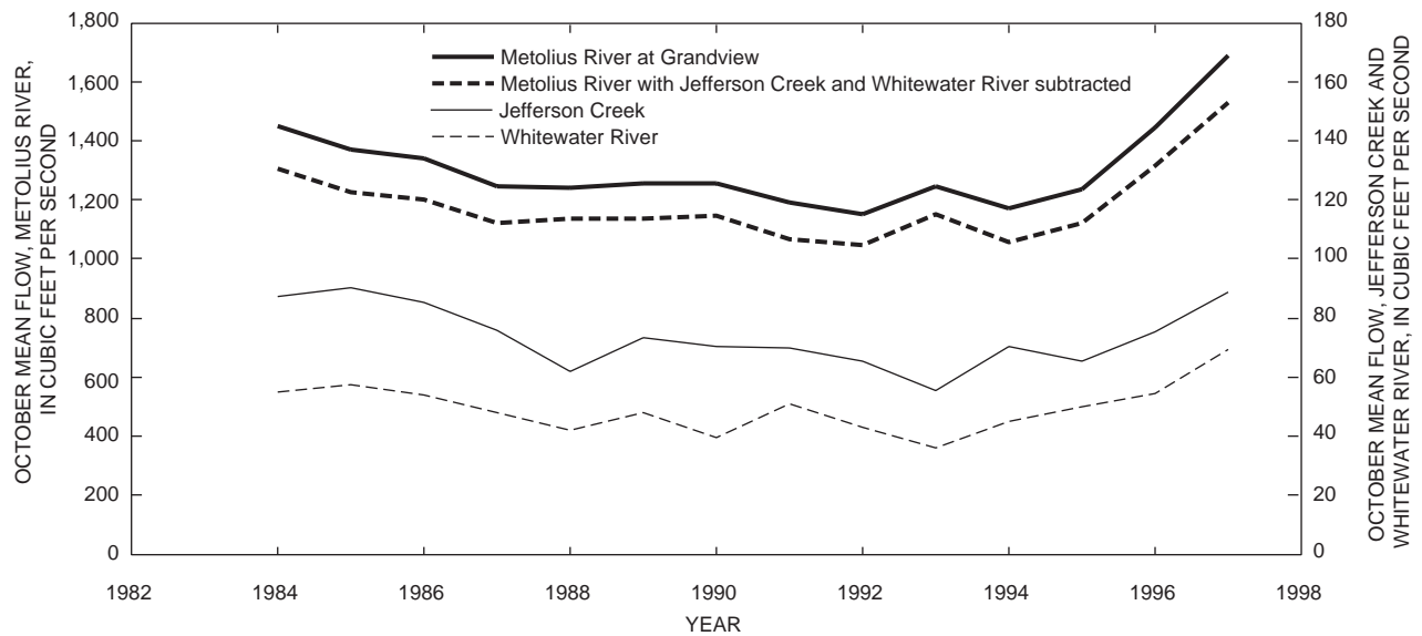
Figure 20. October mean flows of the Metolius River (near Grandview), Jefferson Creek, and Whitewater River, upper Deschutes Basin, Oregon, 1984–97.
