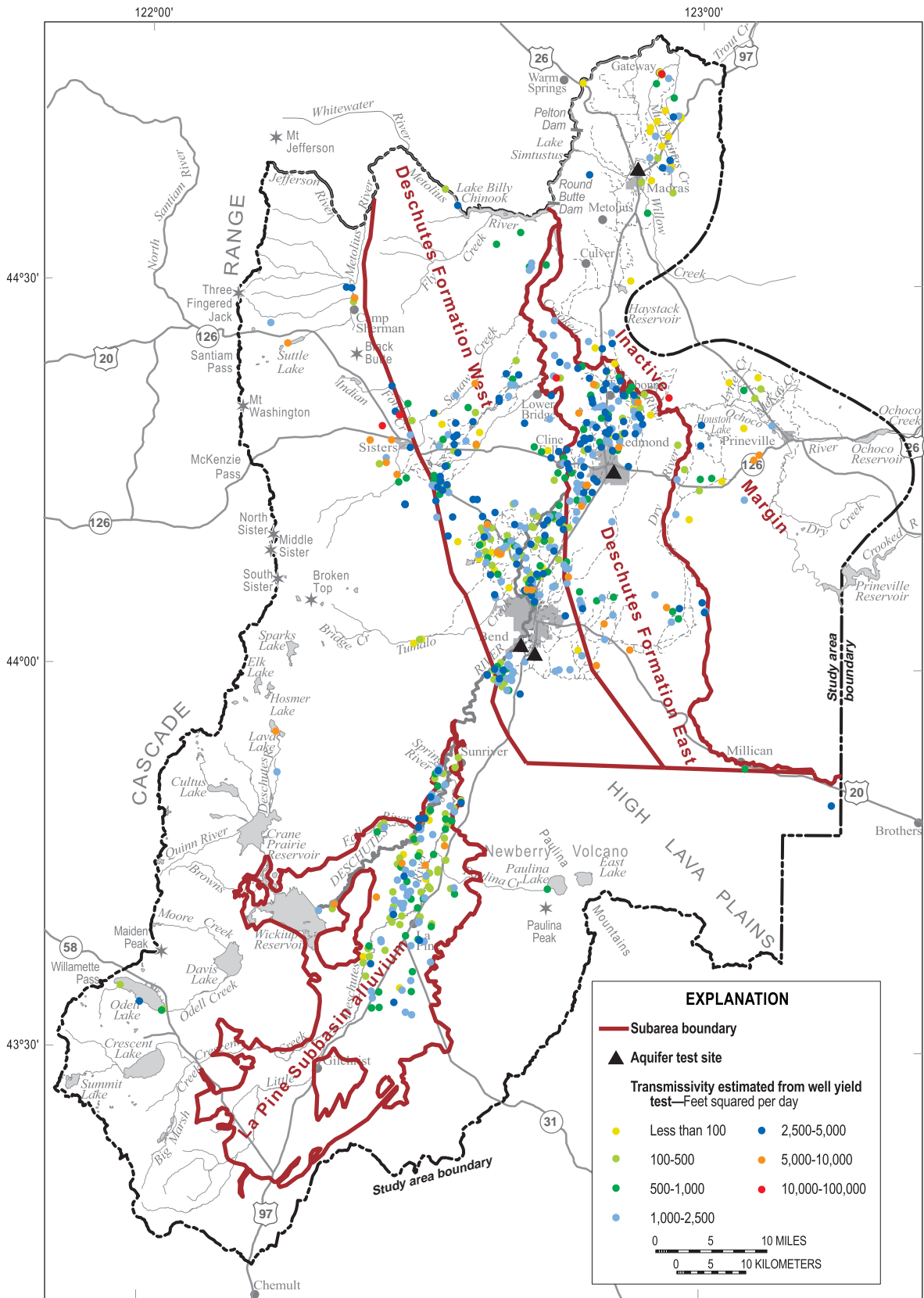
Figure 5. Distribution of transmissivity estimates derived from specific-capacity tests of field-located domestic wells in the upper Deschutes Basin, Oregon, and the locations of aquifer tests conducted for this study.
