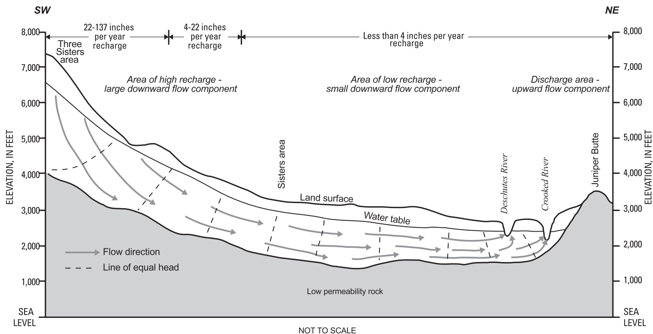
Figure 29. Diagrammatic section southwest-northeast across the upper Deschutes Basin, Oregon, showing flow directions and lines of equal hydraulic head.
