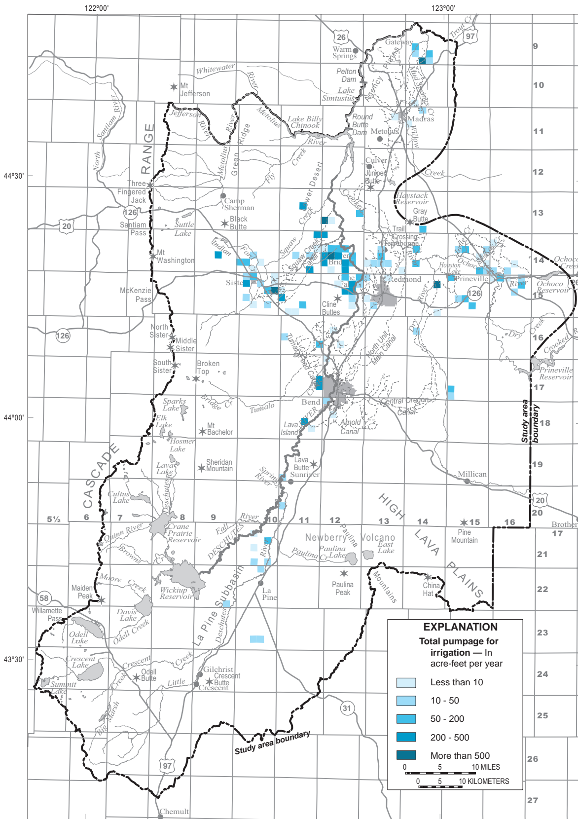
Figure 25. Estimated average annual ground-water pumpage for irrigation in the upper Deschutes Basin, Oregon, 1993–95, aggregated by section.
