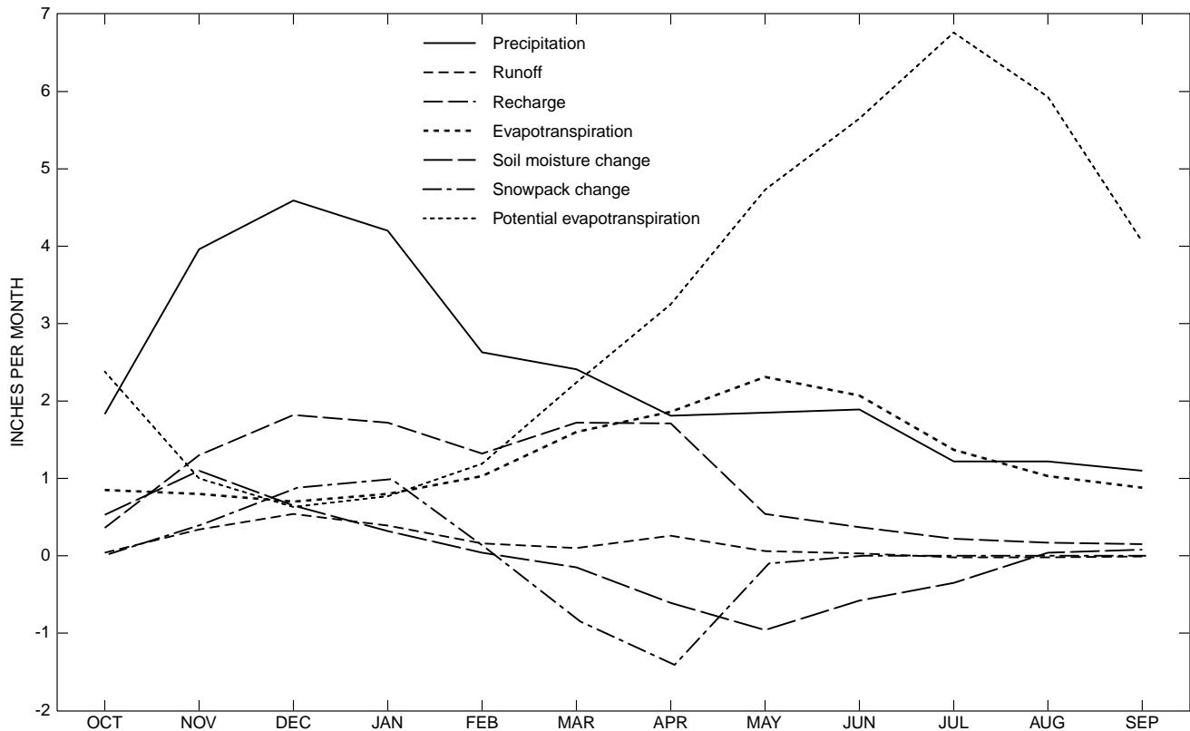
Figure 8. Mean monthly components of the basinwide water budget, estimated using the Deep Percolation Model for water years 1962–97.
