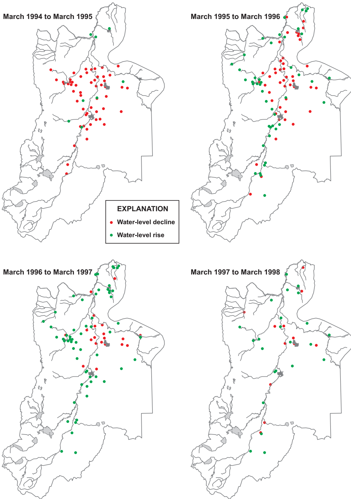
Figure 33. Year-to-year changes in March static water levels in observation wells in the upper Deschutes Basin, Oregon, 1994–98.
