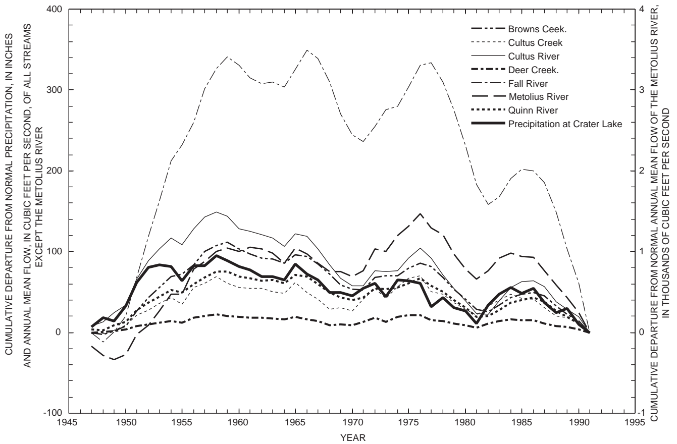
Figure 19. Cumulative departure from normal annual mean flows of selected streams in the upper Deschutes Basin, and cumulative departure from normal annual precipitation at Crater Lake, Oregon, 1947–91.
