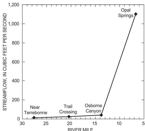
Figure 16. Gain in flow of the lower Crooked River, Oregon, due to ground-water discharge between river miles 27 and 7, July 1994.
