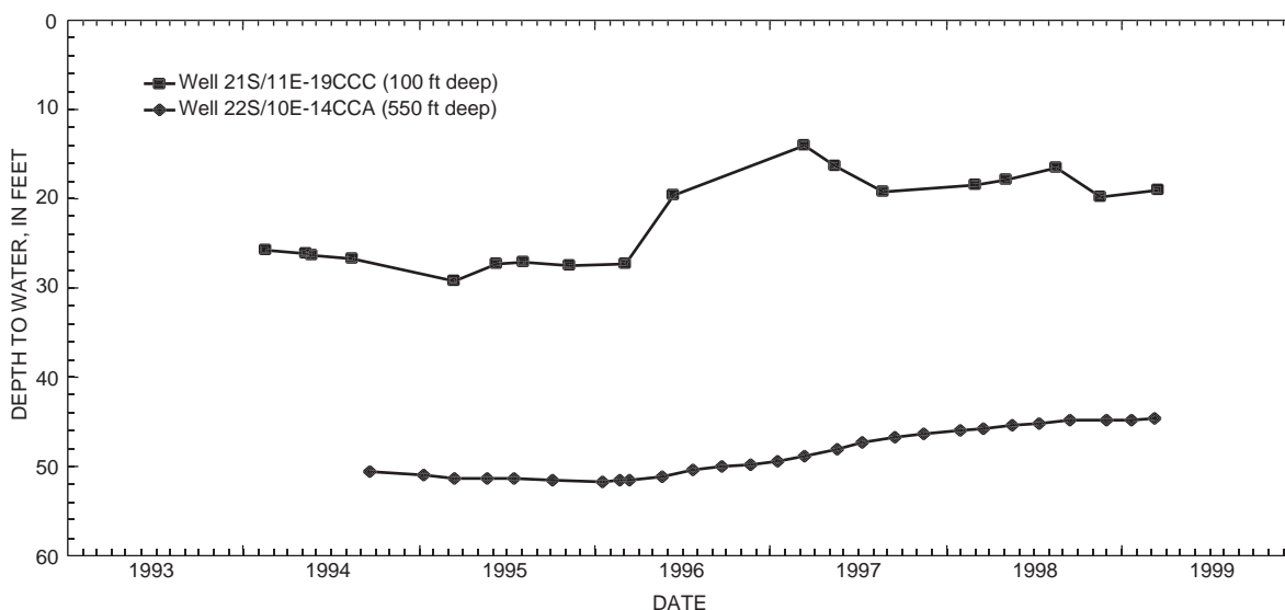
Figure 34. Static water-level variations in a shallow well and a deep well in the La Pine subbasin, Oregon.
