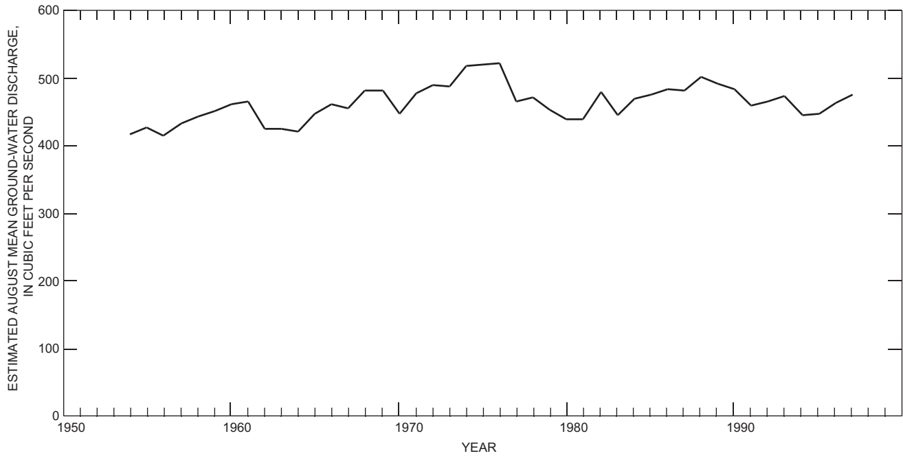
Figure 21. Approximate August mean ground-water discharge to the middle Deschutes River between Bend and Culver, based on the difference between August mean streamflows at gages below Bend and near Culver, 1954–97. (Fluctuations are caused by variations in ground-water discharge.)
