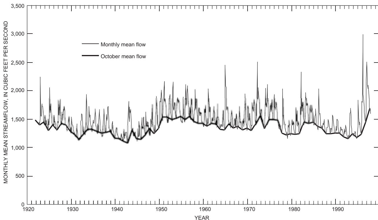
Figure 15. Monthly mean flow of the Metolius River near Grandview. (The line connecting the October mean flows approximates ground-water discharge.)
