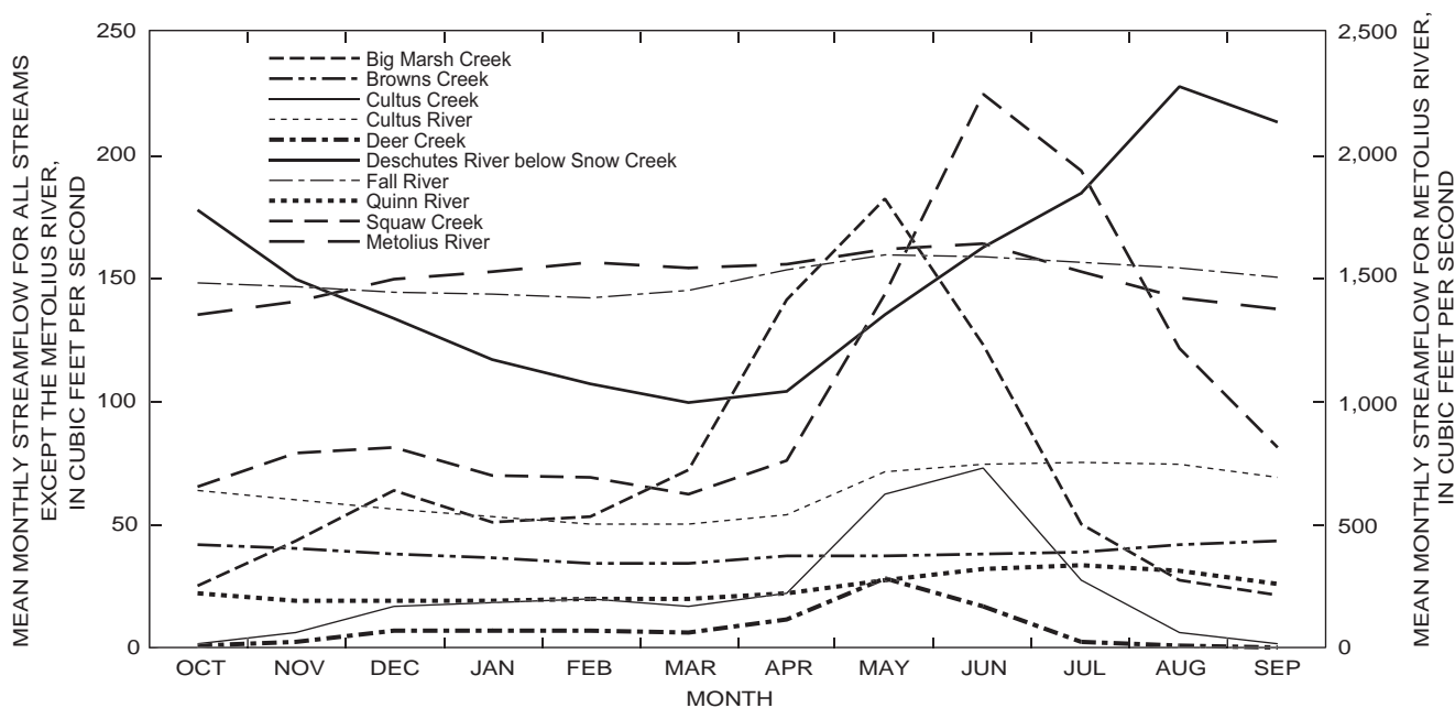
Figure 14. Mean monthly flows of selected nonregulated streams in the upper Deschutes Basin, Oregon.
