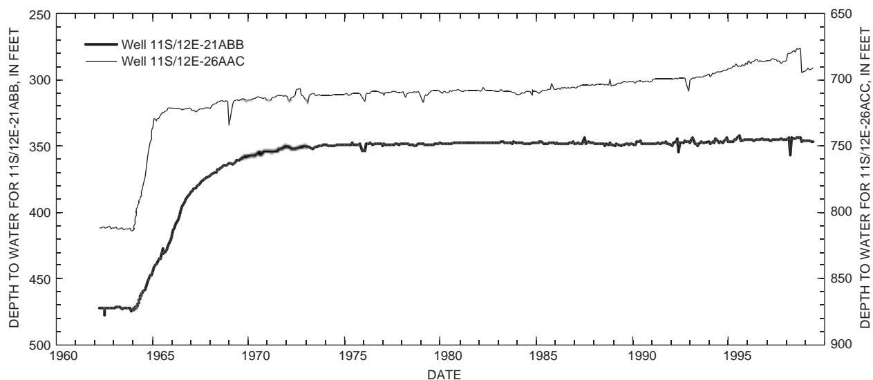
Figure 40. Water levels in two wells near Round Butte Dam, showing the rise in ground-water elevations caused by the filling of Lake Billy Chinook.
