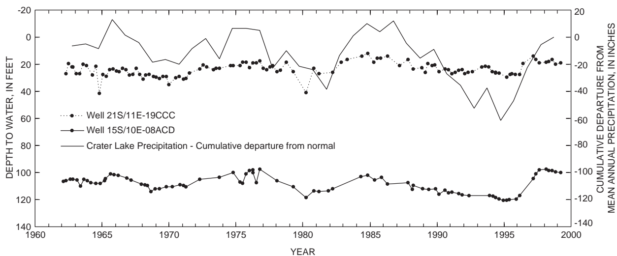
Figure 31. Static water levels in two long-term observation wells in the upper Deschutes Basin, Oregon, and cumulative departure from normal annual precipitation at Crater Lake, Oregon, 1962–98.
