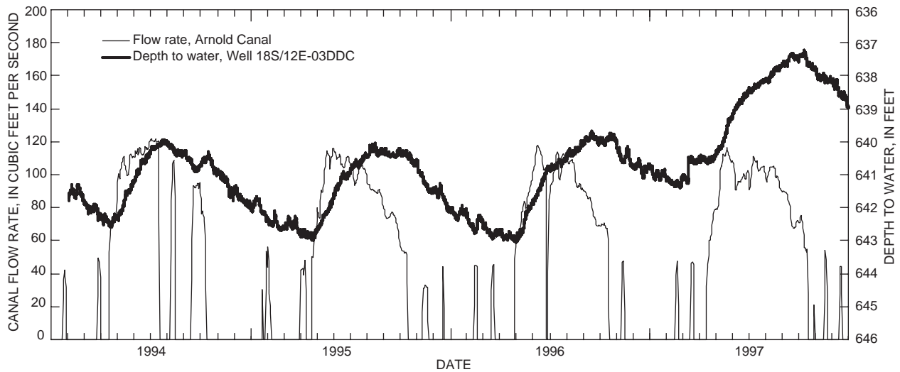
Figure 35. Relation between static water-level variations in a deep well near Bend, Oregon, and flow rate in a nearby irrigation canal.
