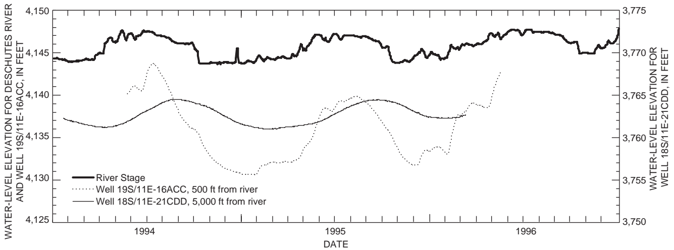
Figure 37. Relation between static water-level variations in two wells at different distances from the Deschutes River and stage of the river at Benham Falls.
