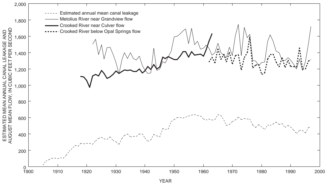
Figure 23. August mean flows of the Crooked River below Opal Springs, the Metolius River near Grandview, and estimated annual mean leakage from irrigation canals, 1905–97.
