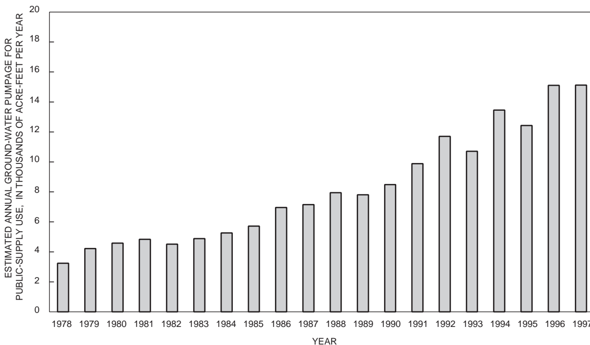
Figure 26. Estimated annual ground-water pumpage for public-supply use in the upper Deschutes Basin, Oregon, 1978–97. (Gross pumping figures do not represent actual consumptive use; a significant proportion of the pumped water returns to the ground-water system.)
