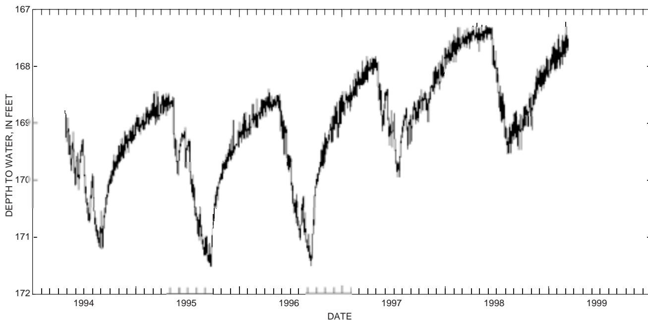
Figure 39. Static water level in an unused irrigation well near Lower Bridge (14S/12E-09ACB), showing seasonal pumping effects from nearby irrigation wells and long-term climatic effects.
