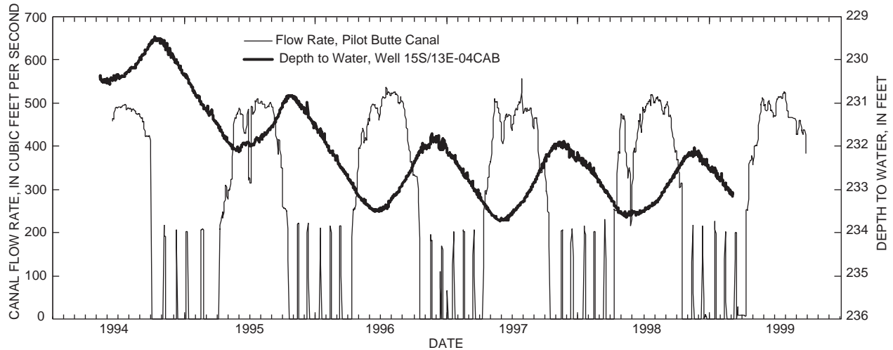
Figure 36. Relation between static water-level variations in a well near Redmond, Oregon, and flow rate in a nearby irrigation canal.
