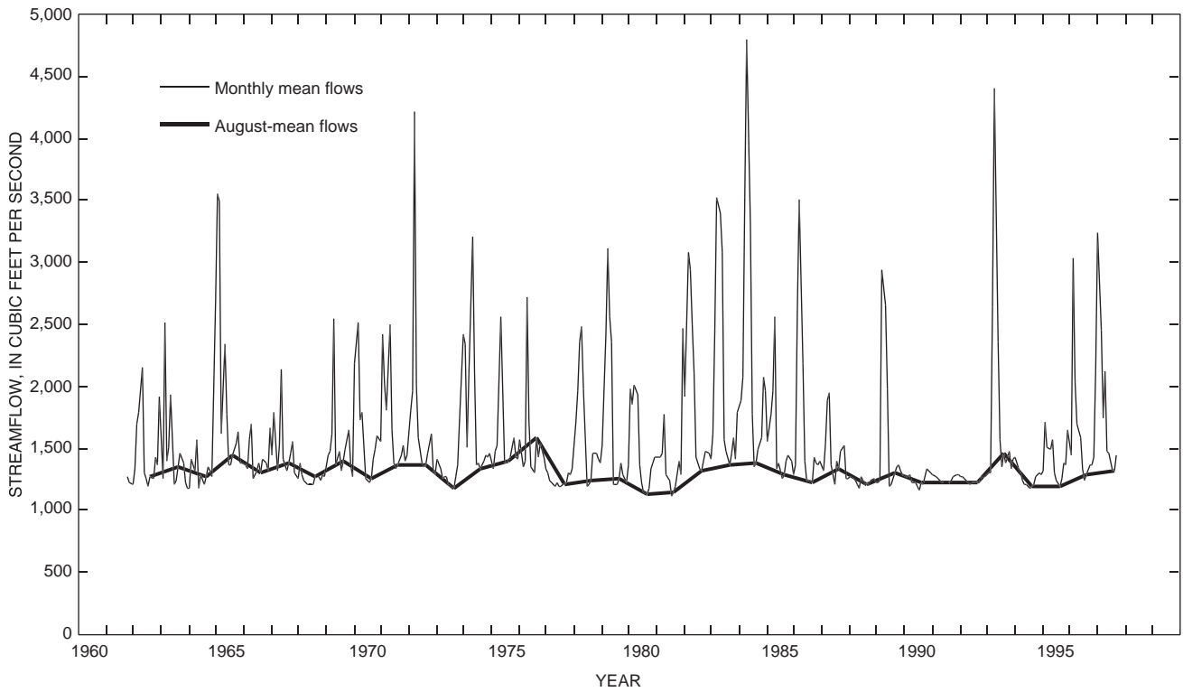
Figure 22. Monthly mean flows of the Crooked River at the gage below Opal Springs, 1962–97. (The line connecting August mean flows approximates late-season ground-water discharge.)
