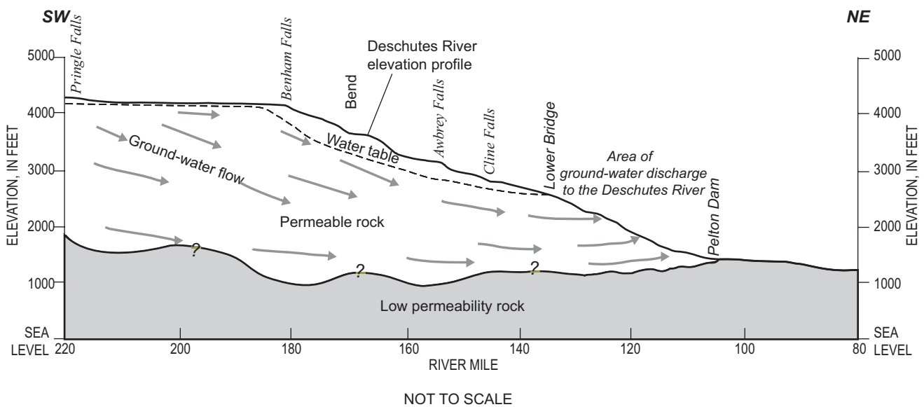
Figure 18. Diagrammatic section showing the effect of geology on ground-water discharge along the Deschutes River upstream of Pelton Dam.
