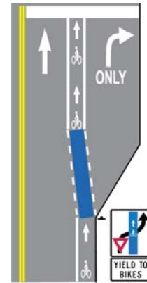
Painted Bike Lane Through Conflict Area
