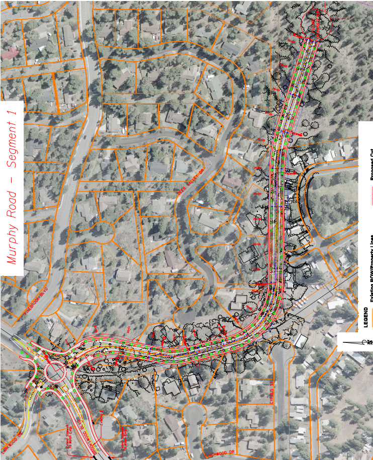
MURPHY ROAD - SEGMENT 1 DATE: 6/9/2008 10:54:25 AM SCALE: 1" = 50' H 1" = 10' V
