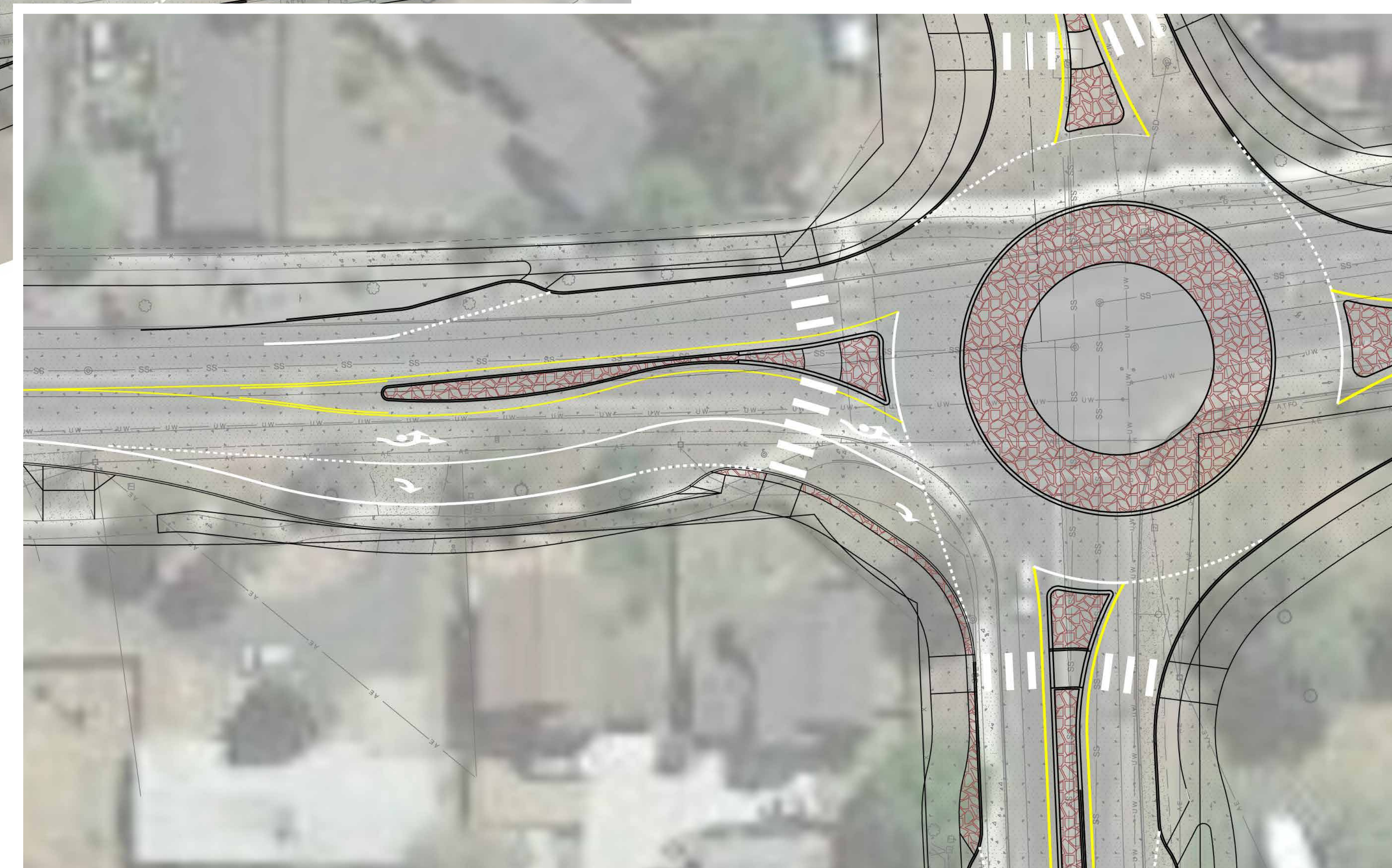
POTENTIAL FUTURE ROUNDABOUT CONFIGURATION - ADDITIONAL TURN LANE
