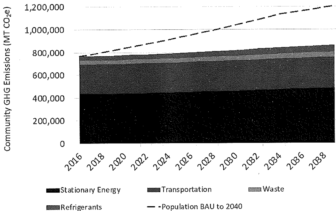
Figure 1: Bend's FY2016 community emissions, by sector, and existing policy forecast to 2040
