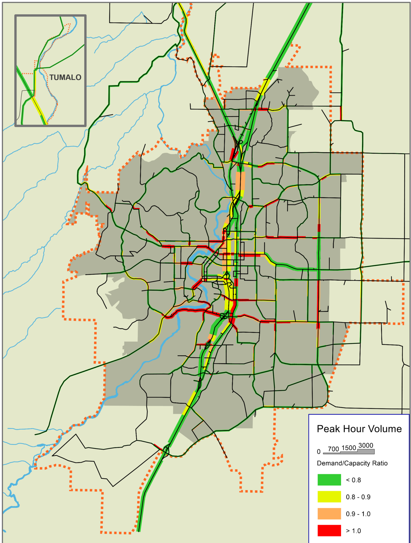
Figure 6-2: 2045 Financially Constrained PM Peak Hour Demand/Capacity Ratios
