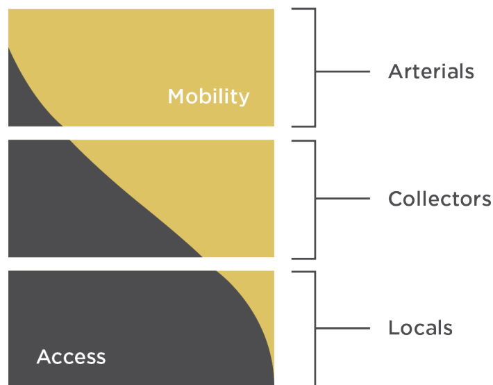
Figure 3-4: Functional Classification of Roadways
