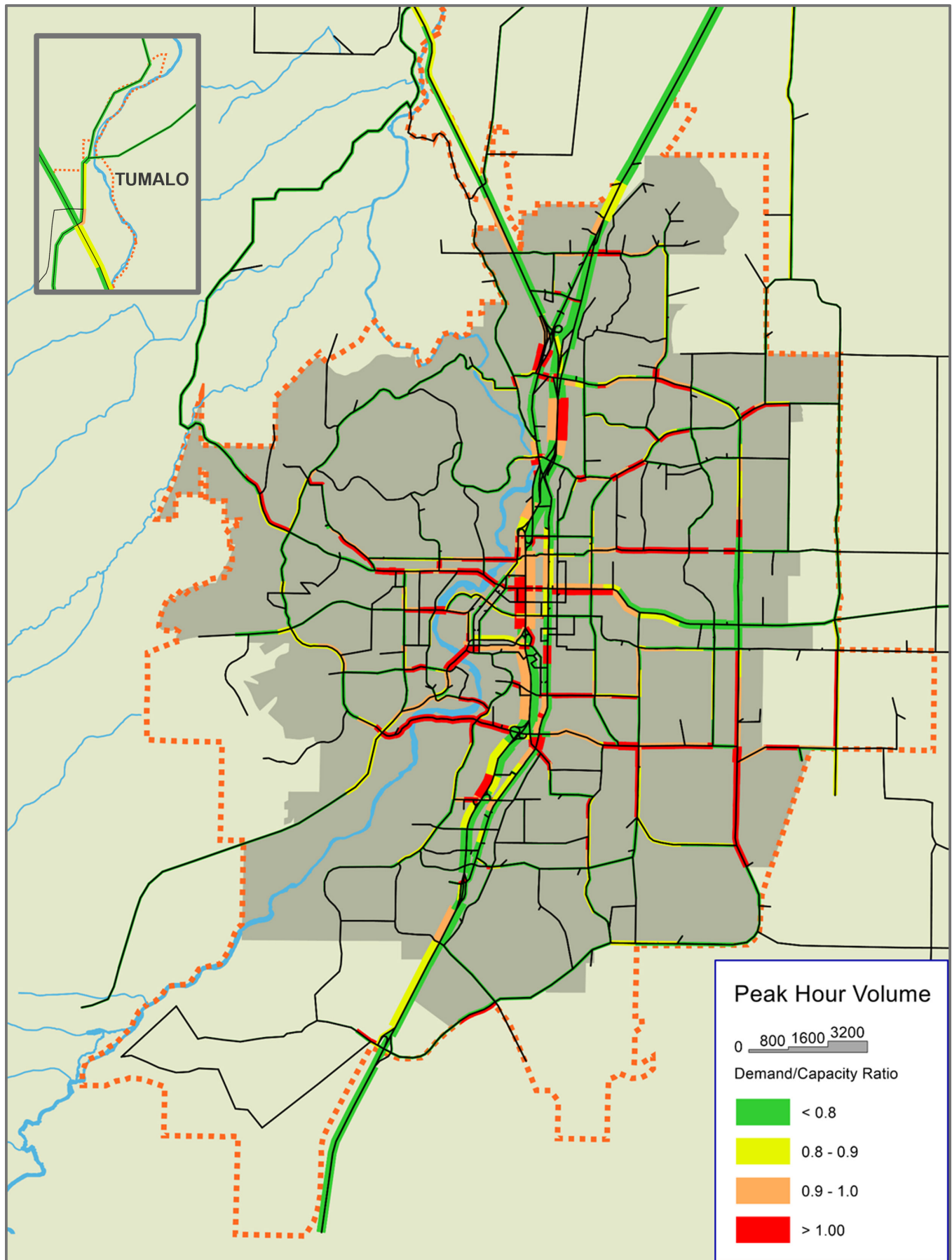
Figure 6-1: 2045 Committed Scenario PM Peak Hour Demand/Capacity Ratios
