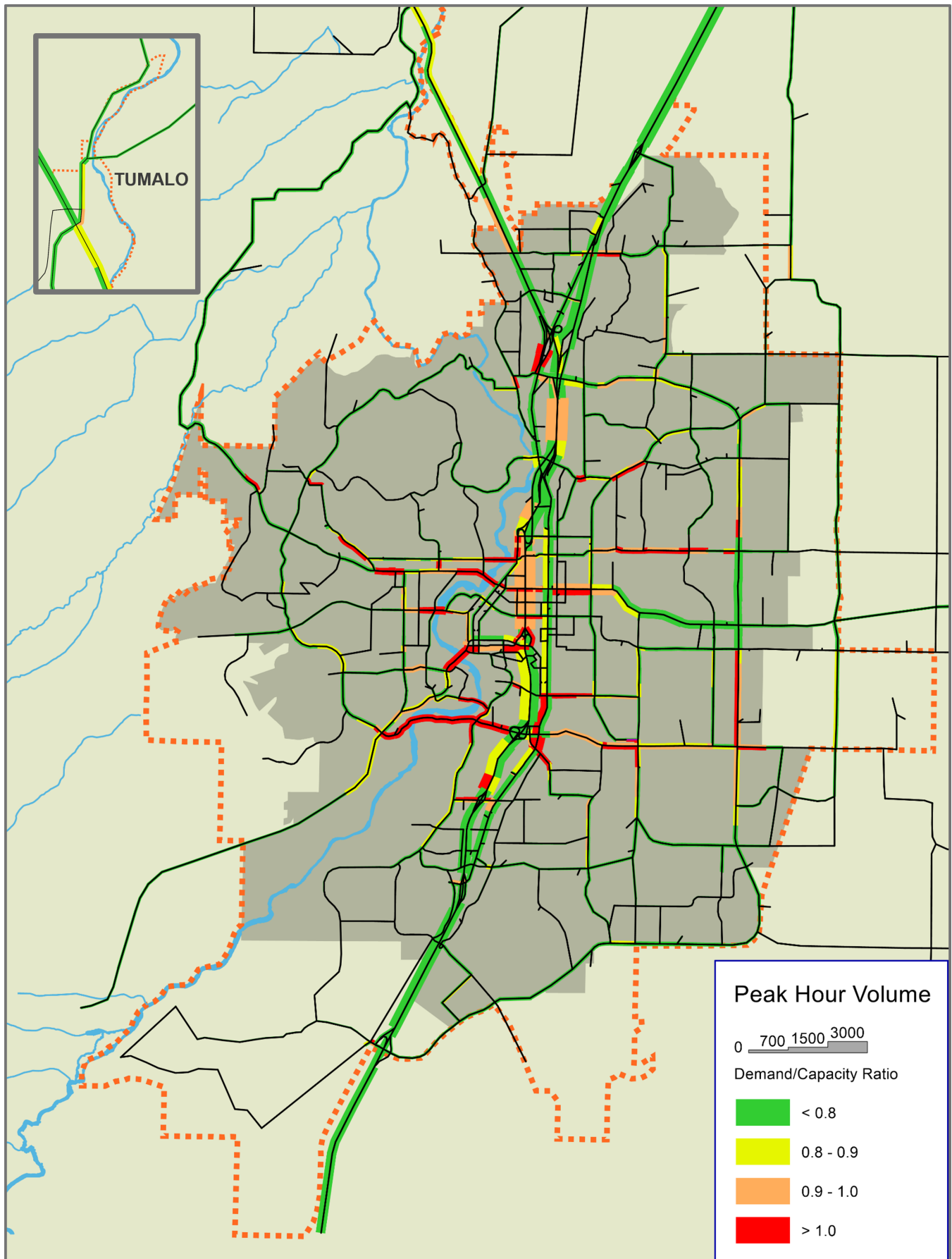
Figure 6-3: 2045 Aspirational Scenario PM Peak Hour Demand/Capacity Ratios
