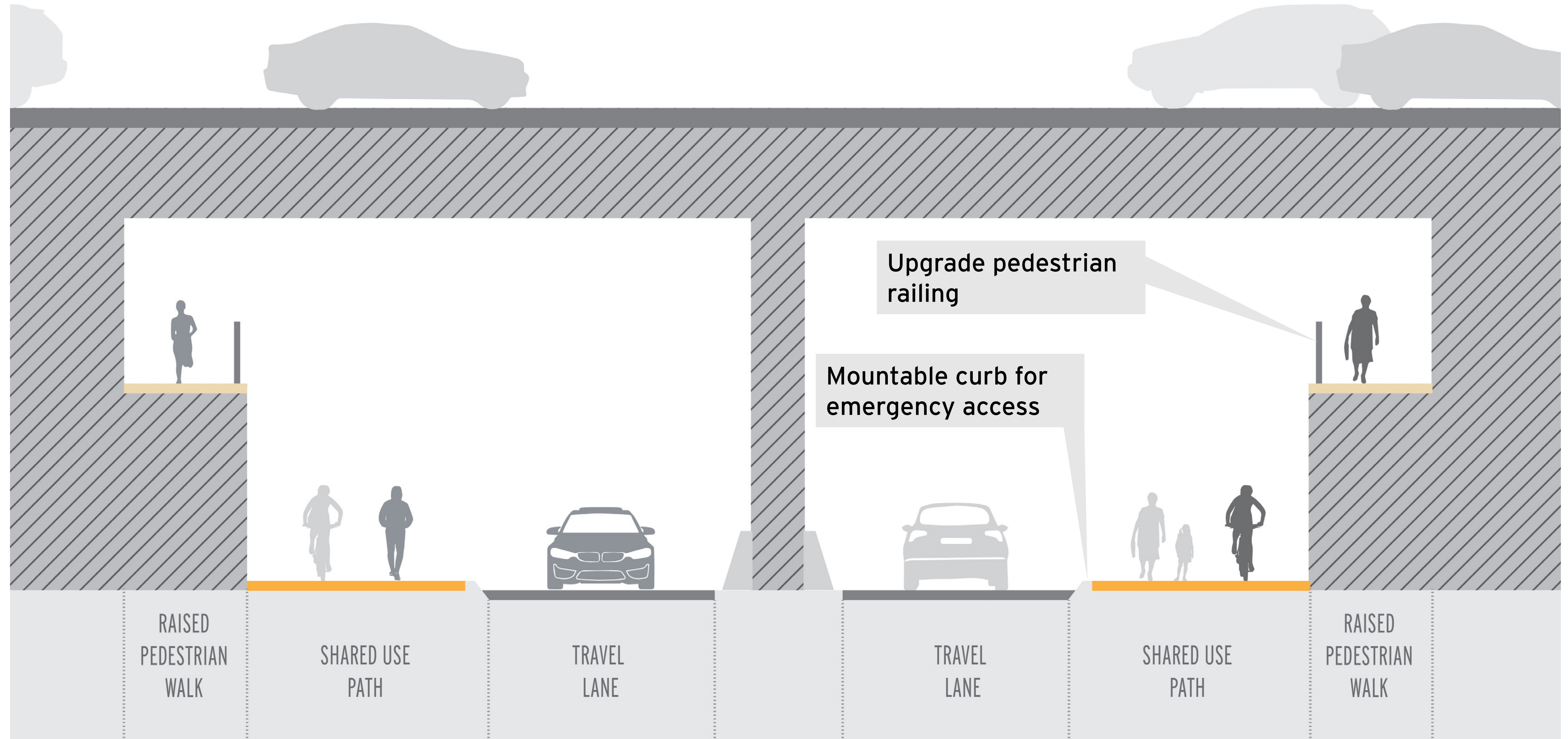
Greenwood Ave: Concept 1 Cross section ©
