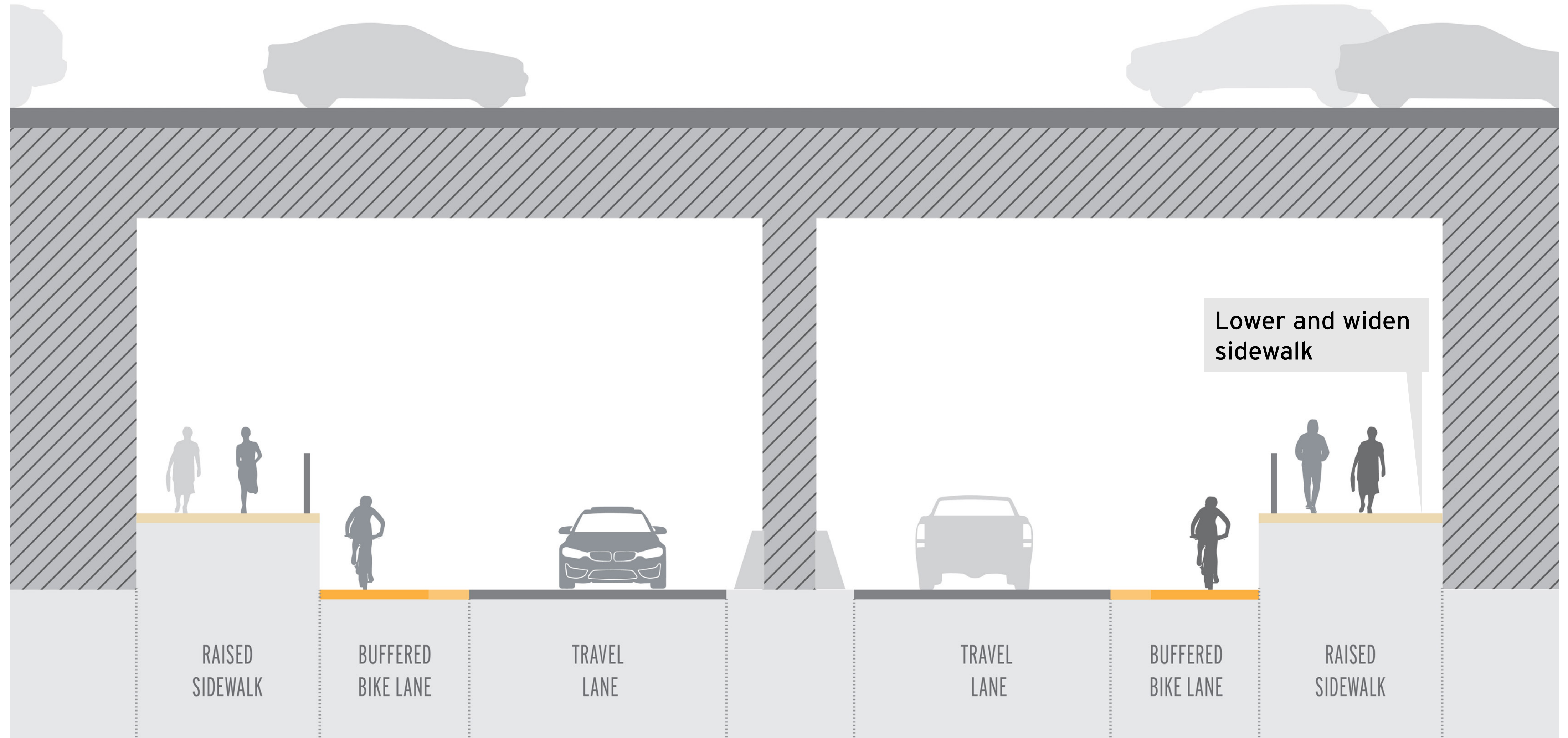
Greenwood Ave: Concept 2 Cross section ©
