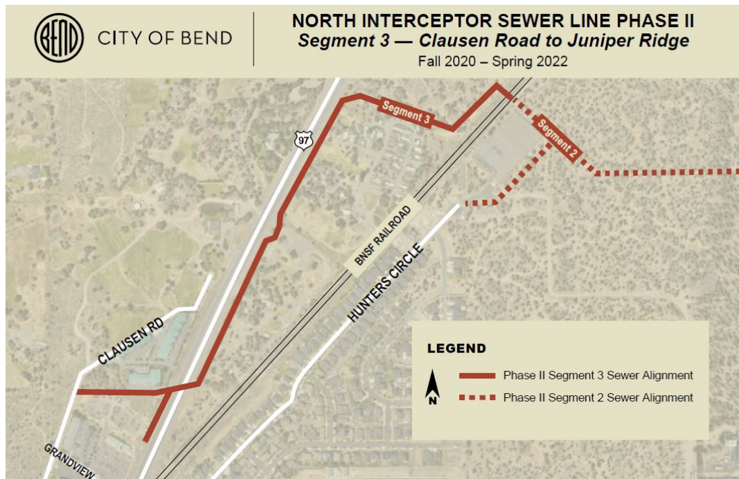
Phase II Segment 3 Sewer Alignment 1
