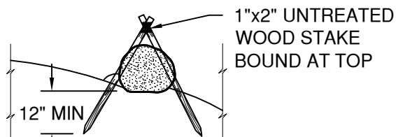
ALTERNATIVE STAKING DETAIL
