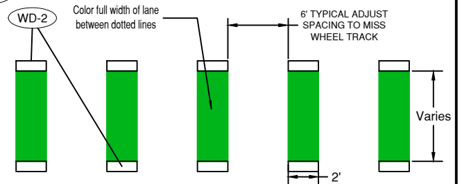
GREEN SUPPLEMENTED BICYCLE LANE DOTTED LINE EXTENSION
