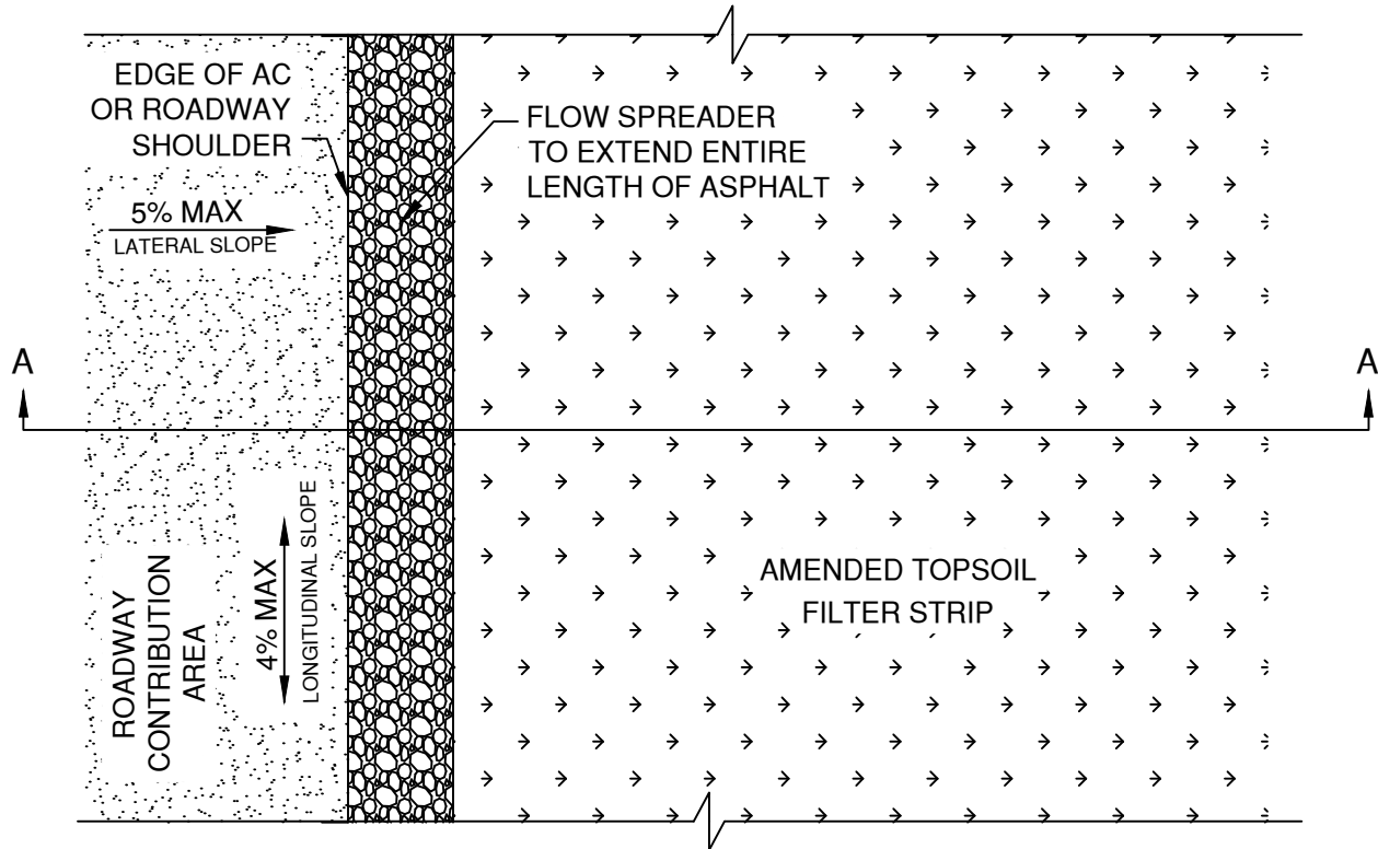
PLAN VIEW
