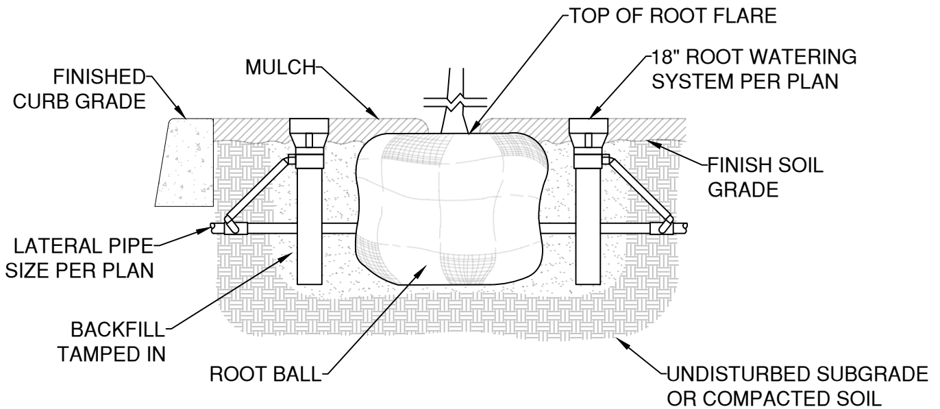
SECTION
