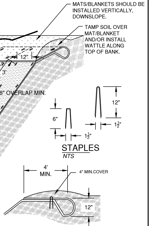
TOP BERM NTS
