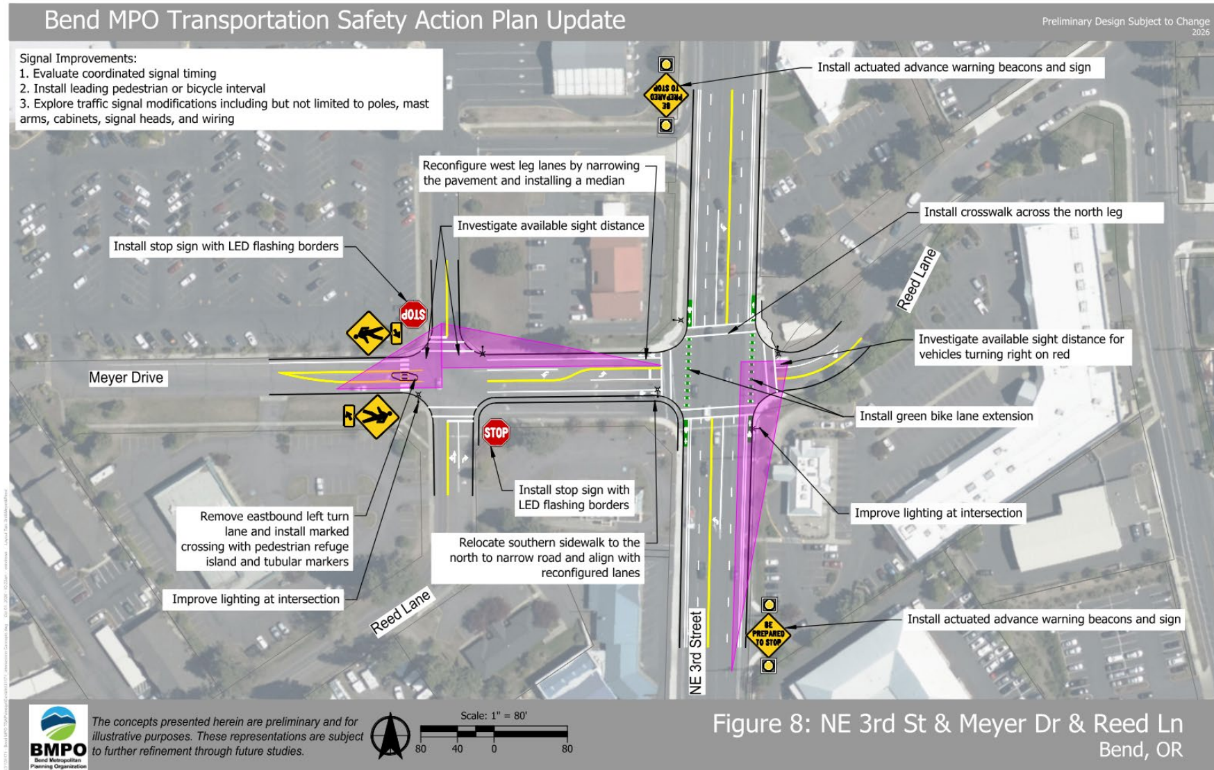
Figure 8. 3rd Street / Meyer Drive-Reed Lane and Meyer Drive / Reed Lane Treatments
