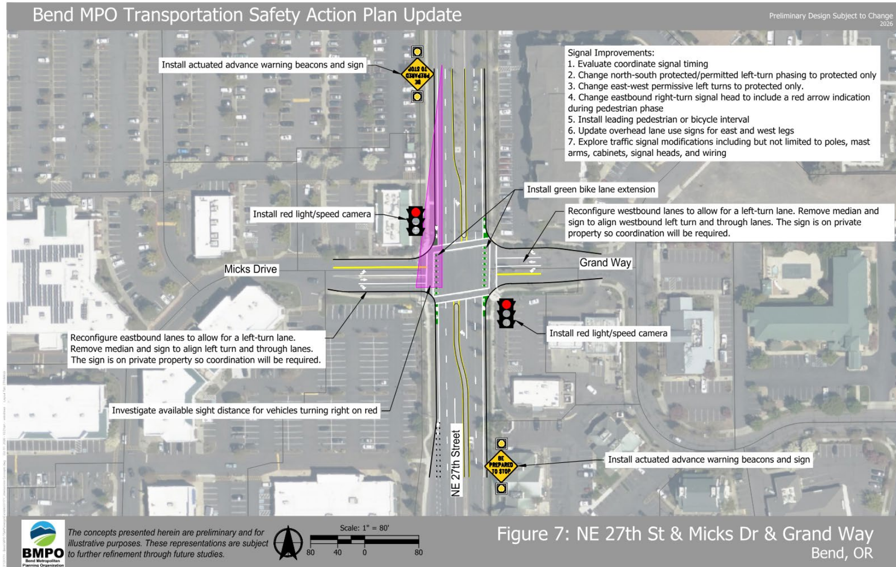
Figure 7. 27th Street / Micks Drive-Grand Way Treatments
