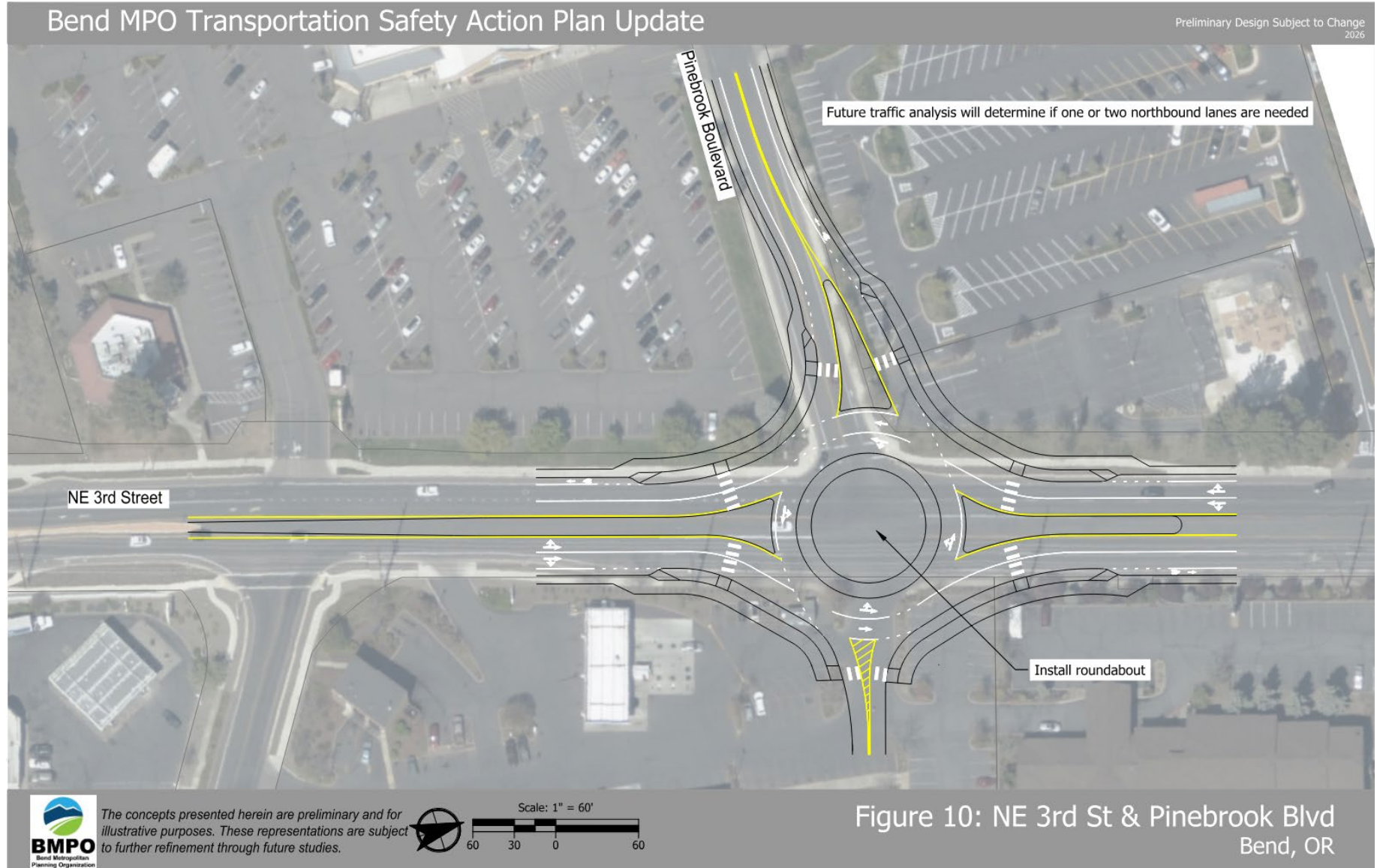
Figure 10. 3rd Street / Pinebrook Boulevard Treatments
