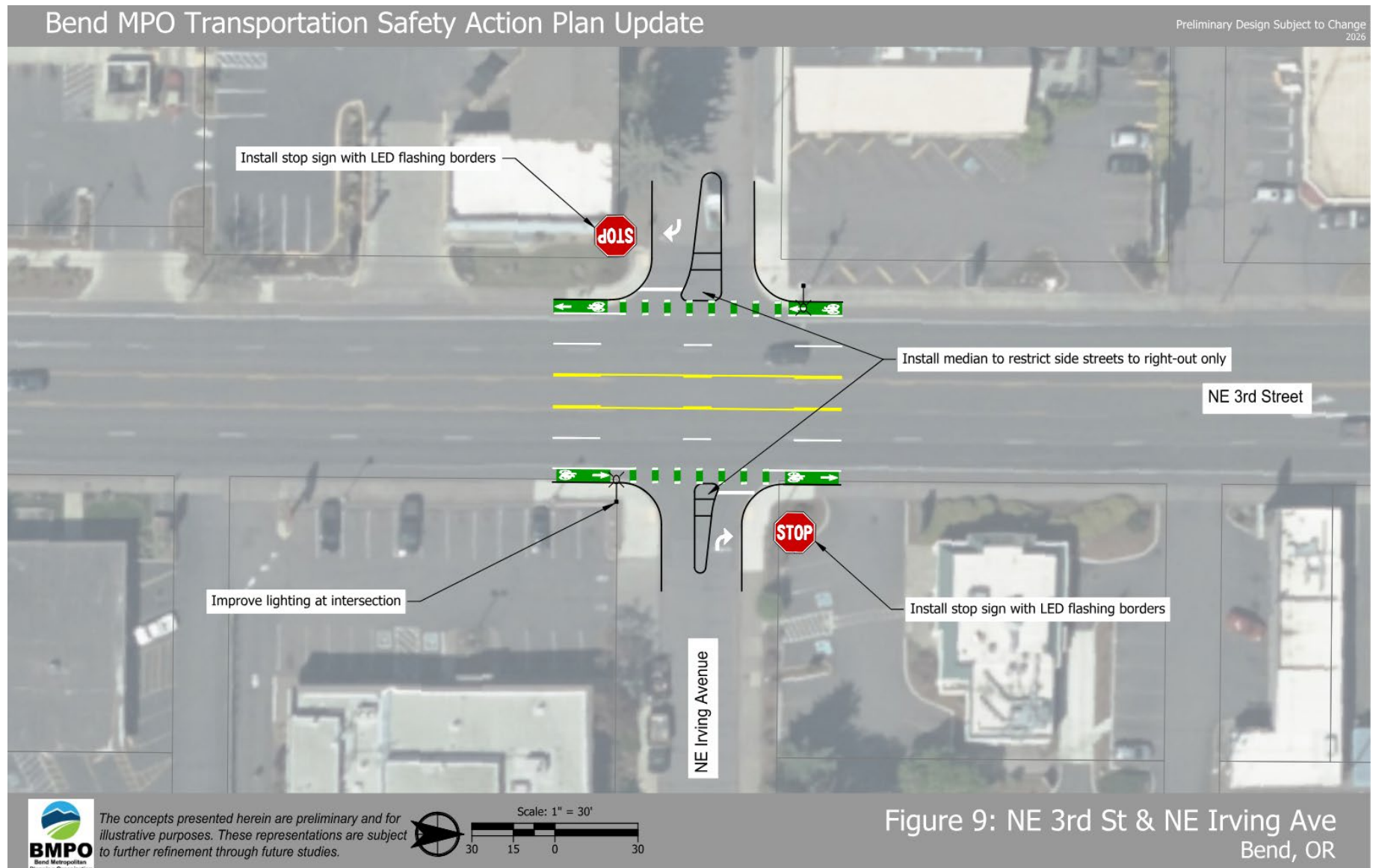
Figure 9. 3rd Street / Irving Avenue Treatments
